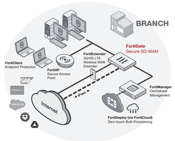
FortiGate 240D-POE deployment in branch office (Secure SD-WAN)
