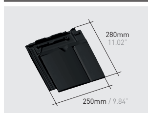
Q100*K | Visum3 right half roof tile klinker
