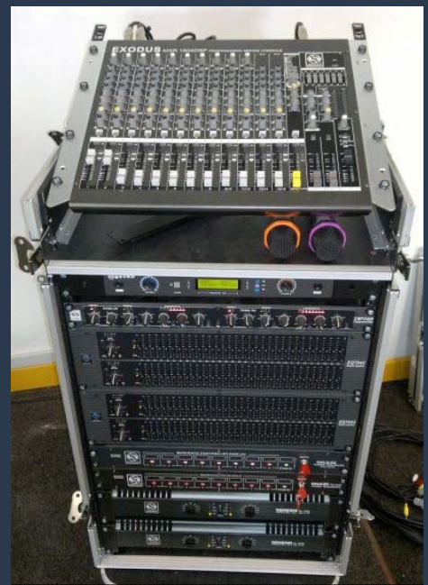
Audio rack for the 8th&9th Floor Theatres
