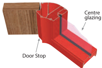
135 / 45 corner post showing Door Stop and Centre Glazing details .
