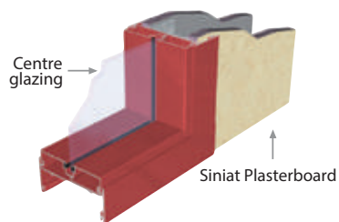
Main Post showing partition board and centre glazing details .
