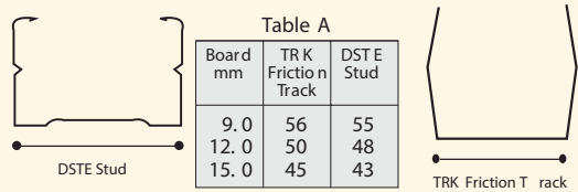
A Dimension of track & stud in relation to board thickness
