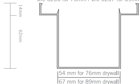
Female Recessed Base Die 6206 for 76mm / Die 6207 for 89mm
